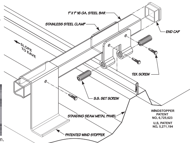
Roof panels utilizing the WINDBAR™ system.
