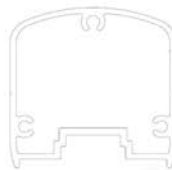
Durarail Square Top Rail (Welded Picket) HEIGHT: 2 5/32" WIDTH: 3 21/32" ALLOY: 6063-T5
