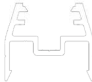
Component Glass Bottom Rail HEIGHT: 1 3/16" WIDTH: 1 5/16" ALLOY: 6063-T5
