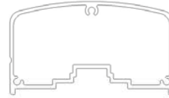
Durarail Port Royal Top Rail (Welded Picket) HEIGHT: 2" WIDTH: 3 1/2" ALLOY: 6063-T5
