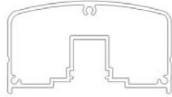
Durarail Port Royal Top Rail (Component Glass) HEIGHT: 2" WIDTH: 3 1/2" ALLOY: 6063-T5
