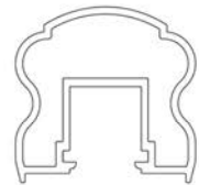
Durarail Heritage Top Rail (Component Glass) HEIGHT: 1 15/16" WIDTH: 2" ALLOY: 6063-T5
