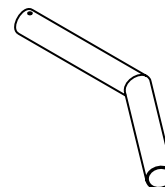
MITERED 143° 12" X 12" (For 37° Stairs)
